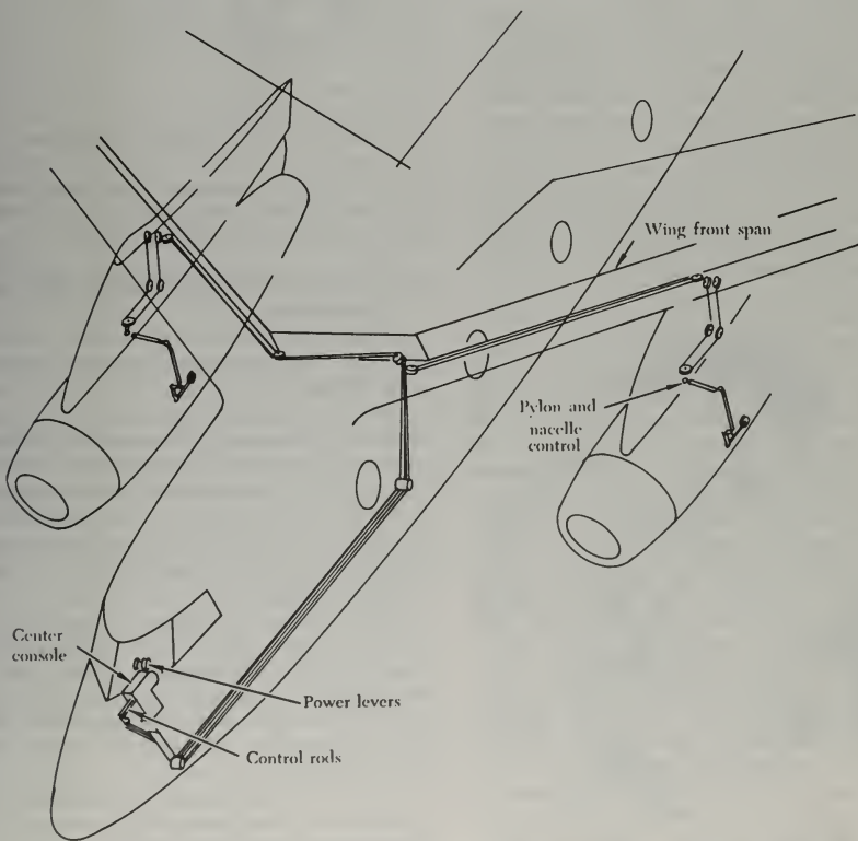
FIGURE 8-20. Power lever control system.
